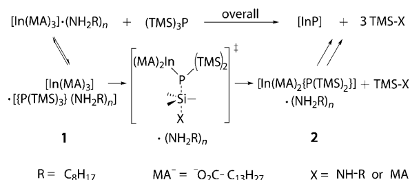
Scheme 1. Proposed mechanistic pathway for amine-inhibited InP synthesis. Both the formation of outer-sphere complex 1 and the irreversible formation of intermediate 2 are inhibited by increased solvation. A charge-dispersion S N 2 transition state for TMS–X bond formation and P–TMS bond cleavage is inferred from the large negative activation entropy and the large rate decrease with added amine.
