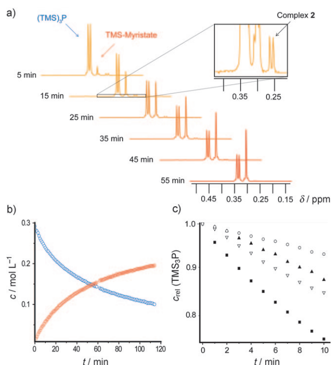
Figure 2. a) Time-resolved ^1\text{H} NMR spectra at 40^\circ\text{C} , showing evolution of (\text{TMS})_3\text{P} (blue) and TMS-MA signals (red) during standard conditions for InP QD synthesis with amines. Inset: Detail of the spectrum at 15 minutes. The doublet at \delta = 0.26 ppm is assigned to 2 . b) Concentration ( c ) profiles of (\text{TMS})_3\text{P} and TMS-MA protons determined at 1 min intervals by integration of spectra represented in Figure 2a. c) Concentration profiles of (\text{TMS})_3\text{P} for InP QD syntheses with varying amine concentrations at 40^\circ\text{C} , normalized at t = 0 . [amine]/[In]: \circ 36:1, \blacktriangle 18:1, \nabla 12:1, \blacksquare 6:1. Reaction rate decreases with increasing amine concentration; reactions without amines reach completion too rapidly to be resolved with our method.
