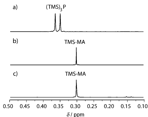
Figure 1. ^1\text{H} NMR spectra of a) (\text{TMS})_3\text{P} at 20^\circ\text{C} before injection, b) the reaction mixture of \text{In}(\text{MA})_3 and (\text{TMS})_3\text{P} in [\text{D}_8]\text{toluene} three minutes after mixing at 25^\circ\text{C} , and c) the reaction mixture of (\text{TMS})_3\text{P} and 6:1 octylamine/ \text{In}(\text{MA})_3 in 1,2- [\text{D}_4]\text{dichlorobenzene} after heating at 178^\circ\text{C} for one minute. Both (b) and (c) show quantitative conversion of (\text{TMS})_3\text{P} into TMS-MA shortly after the reactions are initiated.
